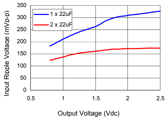
Figure 46. Input ripple voltage for various output voltages with 1 \times 22\mu\text{F} or 2 \times 22\mu\text{F} ceramic capacitors at the input (30A load). Input voltage is 12V.
