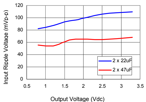
Figure 47. Input ripple voltage in mV, p-p for various output voltages with 2 \times 22\mu\text{F} or 2 \times 47\mu\text{F} ceramic capacitors at the input (30A load). Input voltage is 5V.
